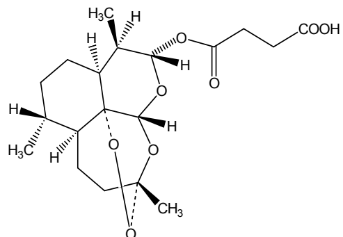
Figure 1. Chemical structures of artesunate and some of its derivatives
